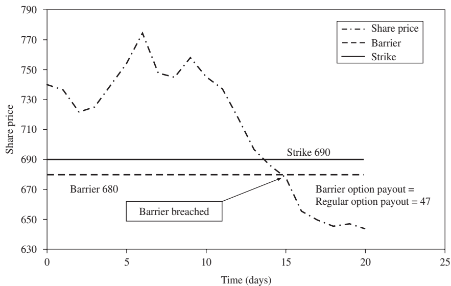
Figure 11.10: Barrier option
