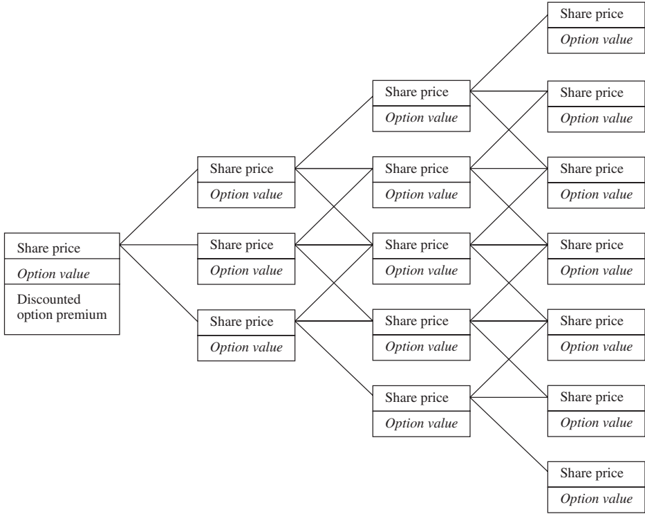
Figure 11.12: Trinomial tree
